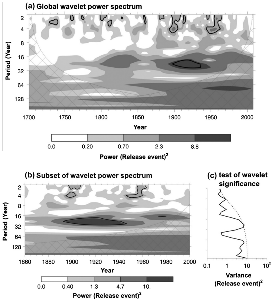
Fig. 5. (a) Wavelet power spectrum of spruce beetle outbreaks for the period 1700–2010. Contour levels represent the proportion of wavelet power above 75%, 50%, 25%, and 5% above each level, respectively. The cross-hatched region is the cone of influence, where zero padding has reduced the variance. Black contour is the 5% significance level, using a red-noise background spectrum. (b) Subset of the reconstructed period (1860–2000) in which the spectral peak of 21.5 years is significant at the 5% level. (c) The global wavelet power spectrum (black line); the dashed line is the significance for the global wavelet spectrum at the 5% significance level (Torrence and Compo, 1998).
