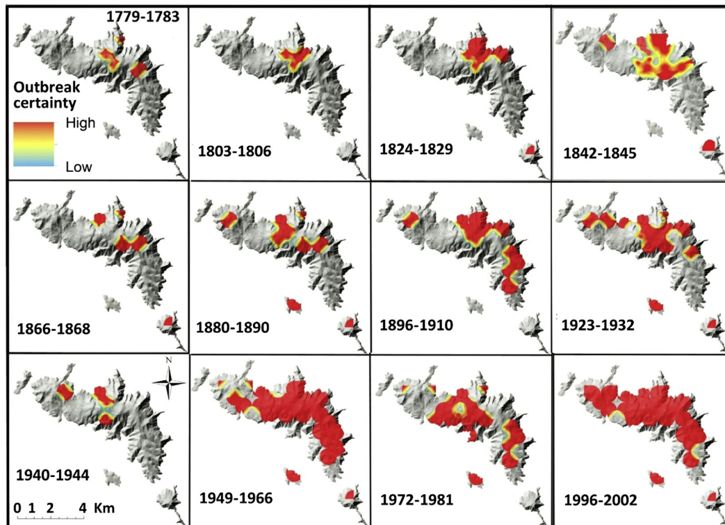
Fig. 6. Spatial progression of spruce beetle outbreaks recorded in 25% or more of sites from 1779 to 1996. Outbreak events are reconstructed from growth releases detected in a minimum of 10% of trees over a five-year period at each of 34 spruce-containing sites. An interpolated outbreak certainty surface is generated from inverse distance weighting of the four nearest point locations with a power function of two at a maximum distance of 750 m (Hessl et al., 2007). The underlying surface is the spruce extent in the Pinaleno Mountains circa 1995.
