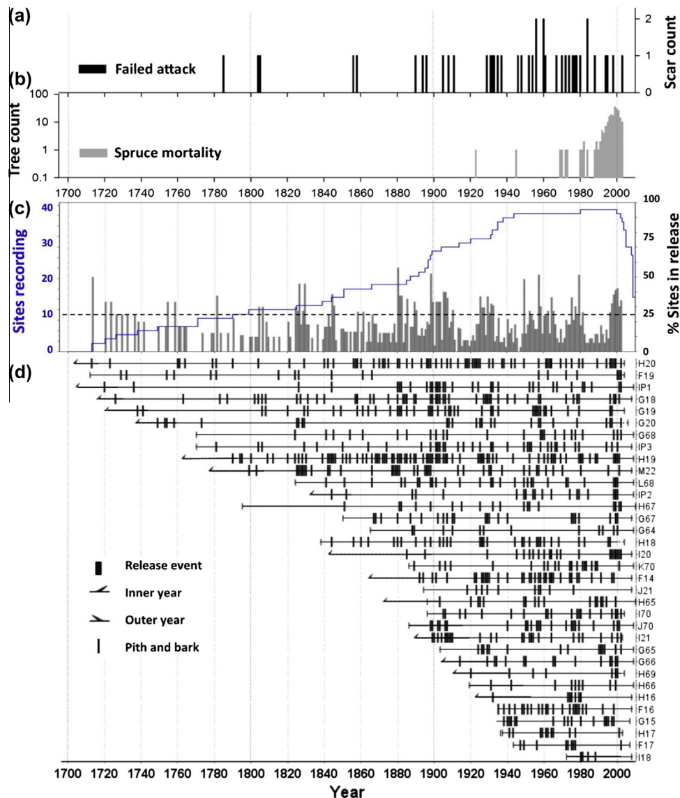
Fig. 4. Multiproxy reconstructions of spruce beetle outbreaks in the Pinaleno Mountains 1700–2008. (a) Bark beetle failed attack scars within individual growth rings of surviving trees. (b) The outer growth ring of beetle-killed trees. (c) Index plot of 34 composited site records recording growth release; the dashed horizontal line intersecting the y-axis to the right indicates 25% of sites in release (used to differentiate outbreaks from other ecological factors). The number of sites recording on the left y-axis is a measure of changing sample depth (spruce occupancy) over time. The earliest growth release attributed to spruce beetle outbreak is in 1779 with nine sites (26% of sites) containing spruce. (d) Site-level record of growth release events occurring in two or more trees over a 5-year period.
