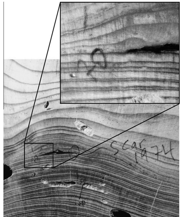
Fig. 2. A scar formed in 1974 from a failed spruce beetle attack on a suppressed understory Engelmann spruce in the Pinaleno Mountains, Arizona. Upper right: magnified image of scar region. From the position of the wound within the ring, it appears that attack occurred early in the growing season, i.e., probably May or June. The failed attack occurred four years prior to the onset of a growth release in 1978.
