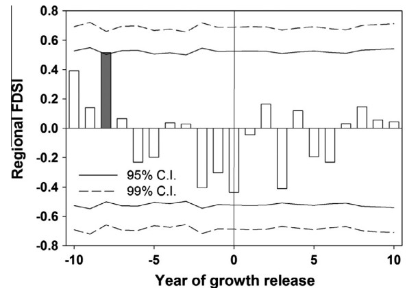
Fig. 8. Association of six spruce beetle outbreaks with regional Forest Drought Severity Index 1770–1896 (Williams et al., 2013). Vertical line at year zero indicates the year for which 25% or more of sites were experiencing growth release. Shaded bars are statistically significant ( p \leq 0.05 ) deviations from the 126-year mean value of FDSI. Confidence intervals of 95% and 99% are indicated by solid and dashed lines respectively.
