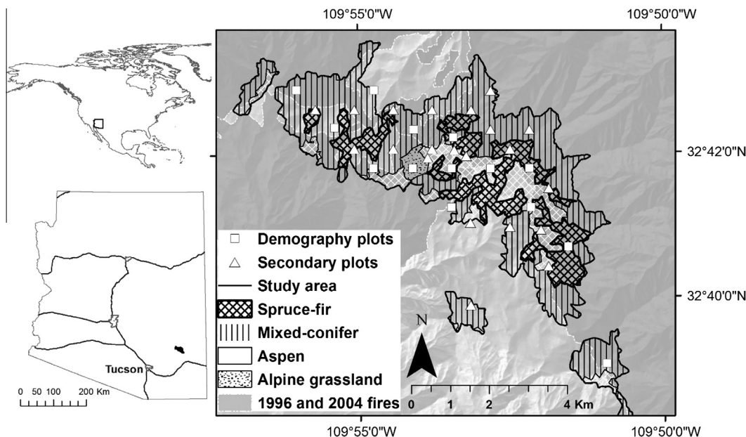
Fig. 1. Location and sampling design of spruce-containing forest in the Pinaleno Mountains, Arizona, USA. Study area denotes elevation above 2835 m. Distributions of forest types are from LANDFIRE biophysical setting generalized to a minimum patch size of 6.75 ha (LANDFIRE, 2013). Fire extents are from the USFS Monitoring Trends in Burn Severity database (MTBS, 2013).
