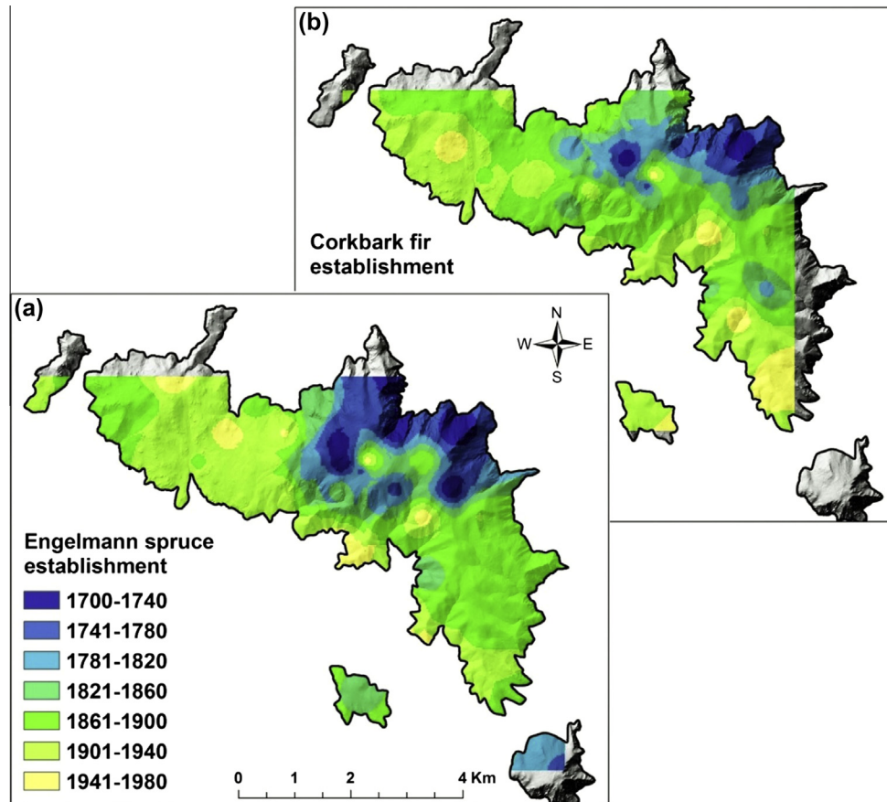
Fig. 3. Temporal progression of Engelmann spruce (a) and corkbark fir (b) tree establishment following stand-replacing fire in 1685. Colors associated with windows of seedling establishment apply to both figures. Interpolated stand age surfaces are generated from inverse distance weighting of minimum tree establishment dates from 44 spruce (a) and 37 corkbark fir (b) gridded point locations. The interpolation algorithm used four nearest point locations with a power function of two.
